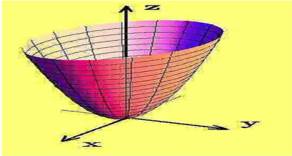
Figure 7-6. Elliptic paraboloid
